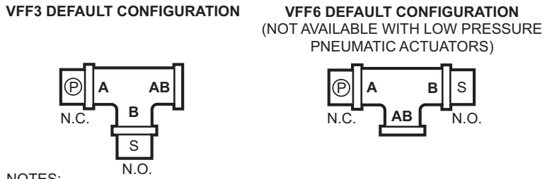
Fig. 11. 3-way VFF3, VFF6 dimensions with 80 psi (high pressure) pneumatic spring return actuators
