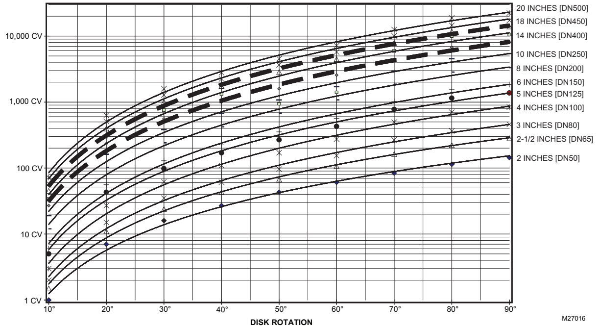
Fig. 13. VFF flow characteristics
