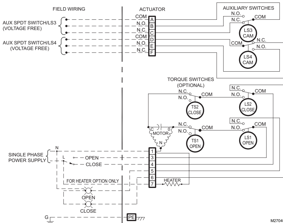
Fig. 26. NEMA 4 floating/2-position industrial-grade actuator for valves 14" to 20" (VFF...4A)
