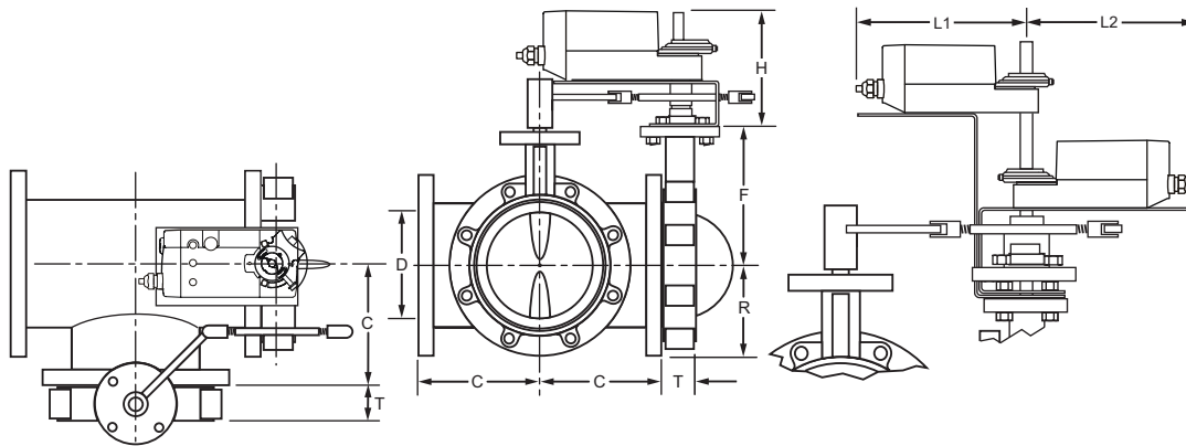
Fig. 2. 2-Way VFF dimensions with NEMA 2 (Honeywell DCA) actuators
