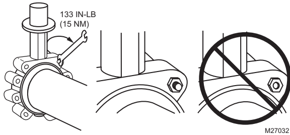
Fig. 20. Flange bolt installation guidelines
